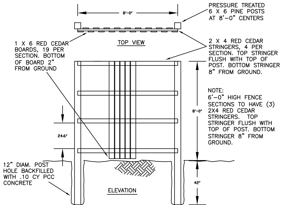
CEDAR FENCE DETAIL
