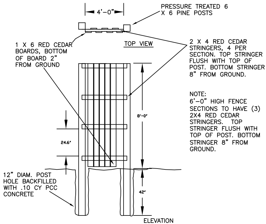
CEDAR GATE DETAIL
